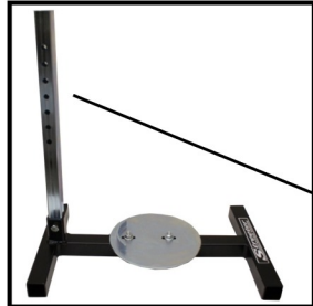
Install vertical post, using 5/16 bolt and nut. Tighten snug.
