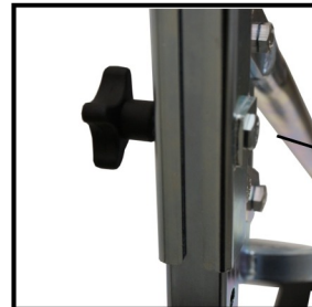
Slide Breaker Handle onto post, using 5/16 bolt and knob. Set height accordingly to your wheel size.
